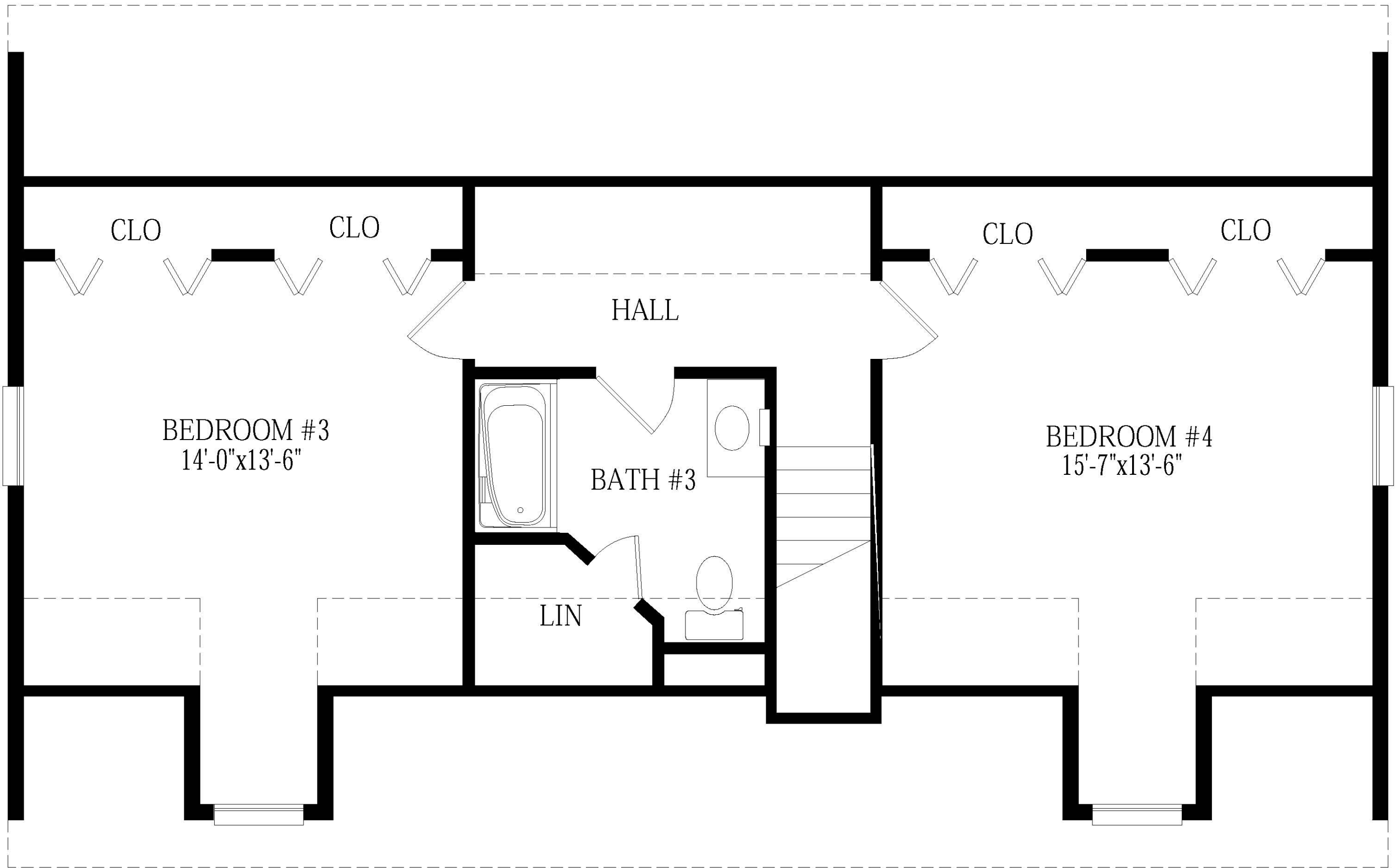
PROPOSED 2ND FLOOR
