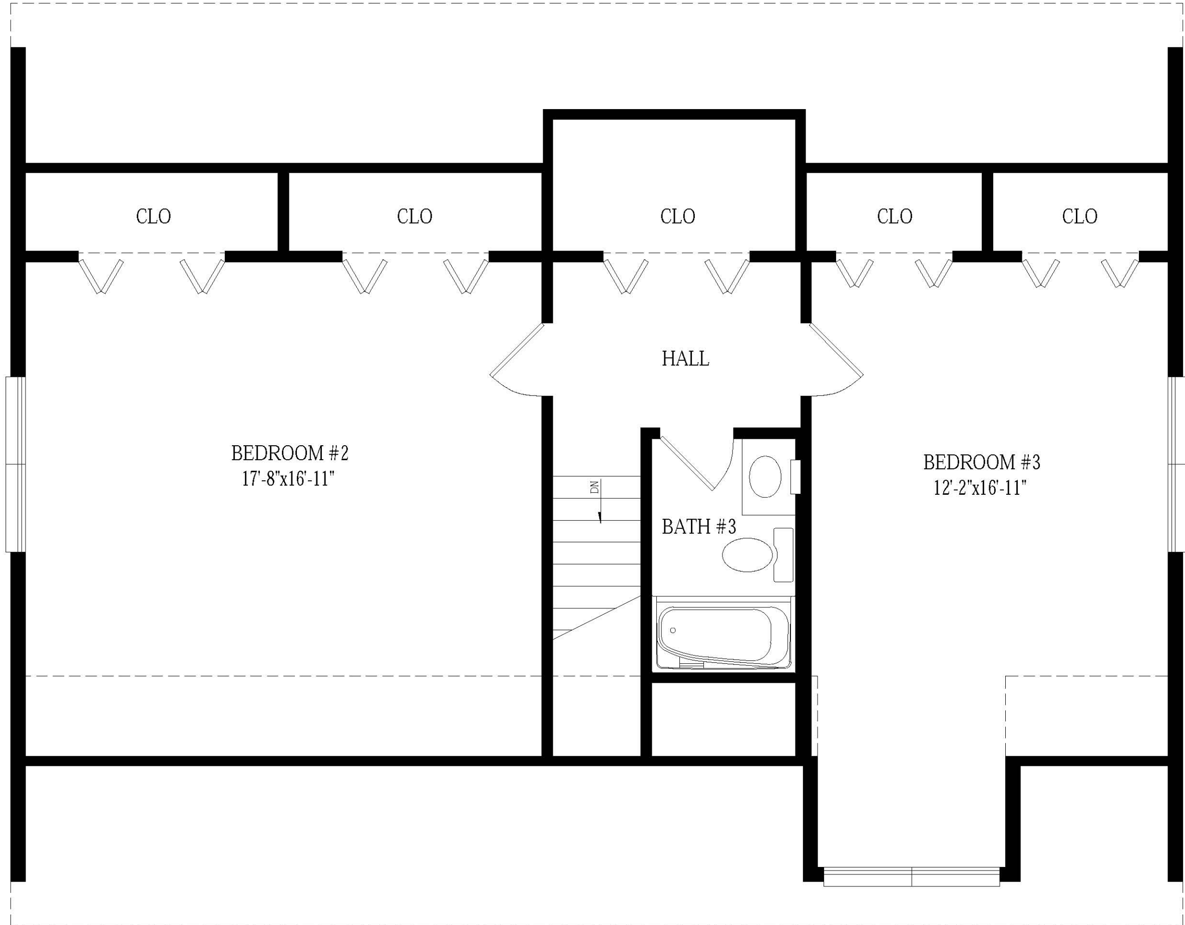
PROPOSED 2ND FLOOR
