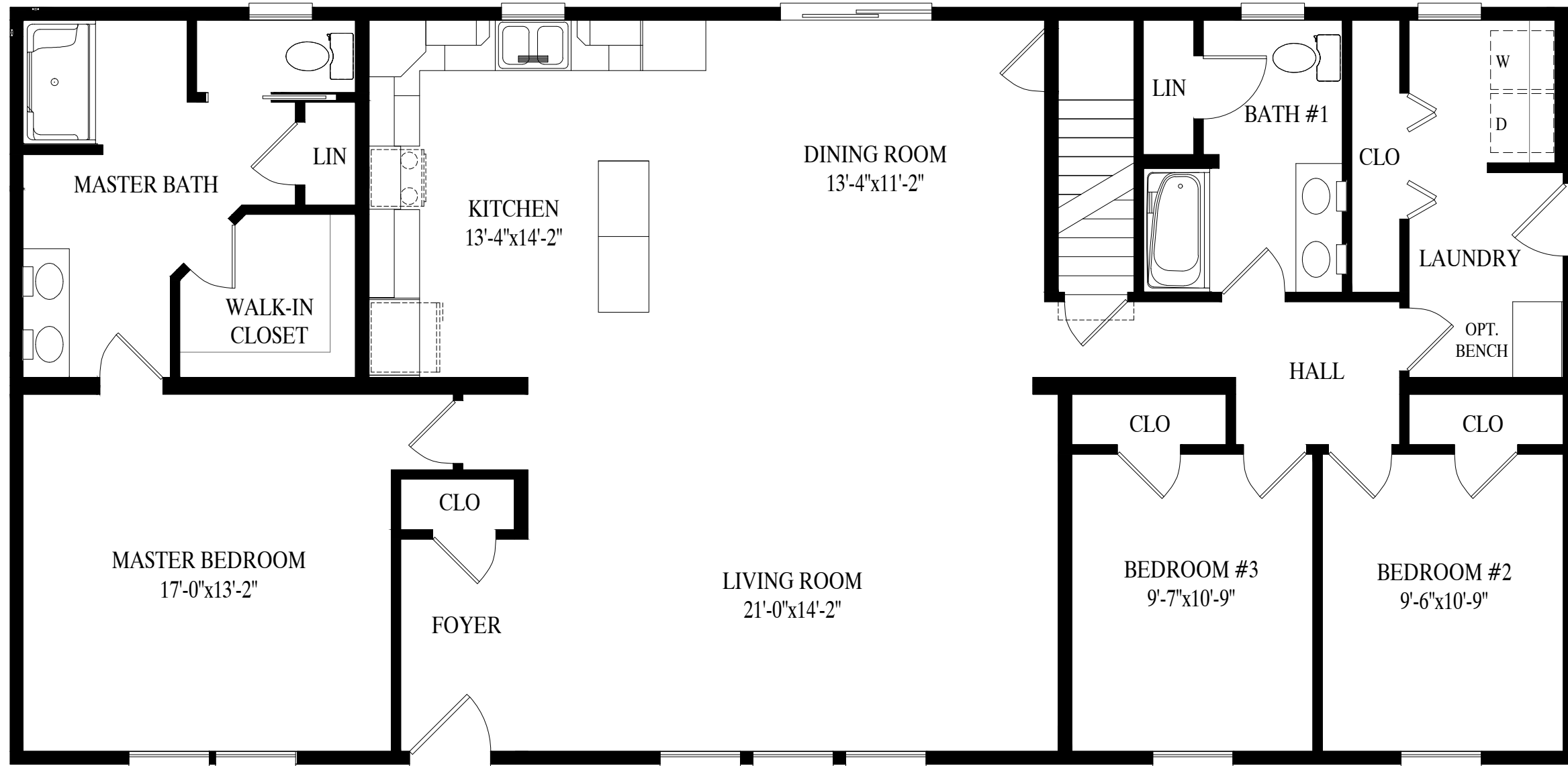
MONTICELLO 30' x 62' 1860 SQ FT
