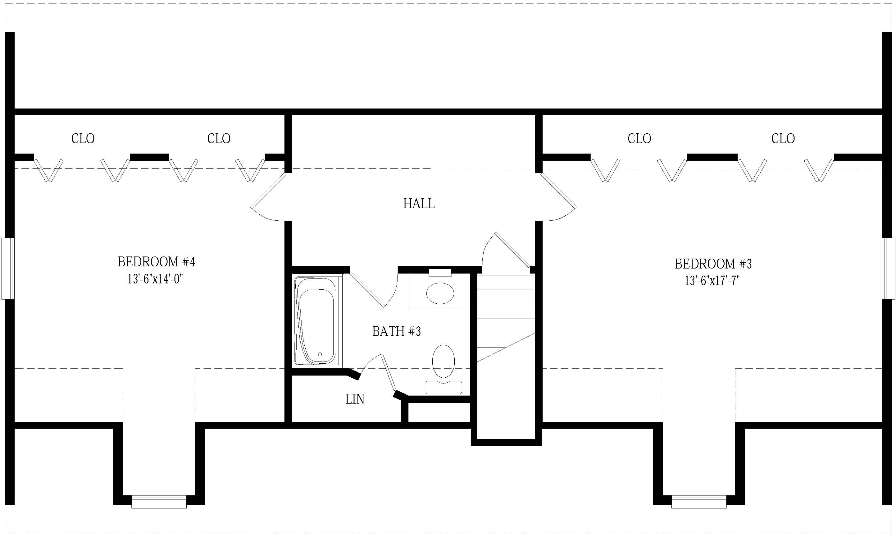
PROPOSED 2ND FLOOR
